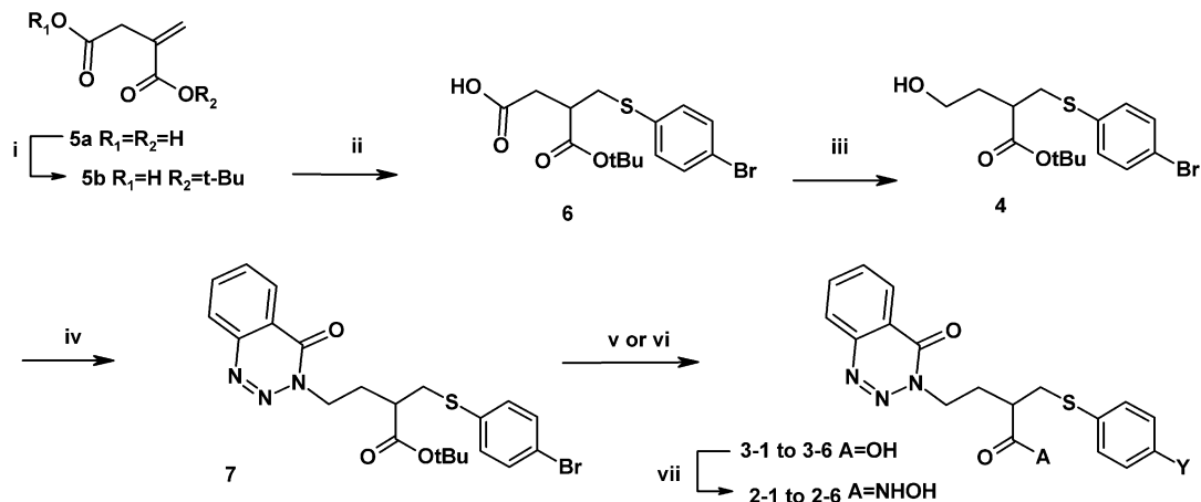
Scheme 3. Synthesis of compounds 2–1 to 2–6 and 3–1 to 3–6 . (i) (a) MeOH, amberlyst-15, rt 80 h, (97%); (b) isobutene, H 2 SO 4 , CH 2 Cl 2 , rt 12 h (67.5%); (c) LiOH, H 2 O/dioxane, 0 °C, 1.5 h, rt, 2 h (75%); (ii) MeONa, MeOH, 4-BrPhSH, rt, 12 h ( 6 , 80%); (iii) (a) ClCO 2 iPr, NMM, DME, 0 °C, + 12 h, rt; (c) NaBH 4 , H 2 O/DME, –10 °C, 1 h, ( 4 , 74%); (iv) PPh 3 , DIAD, benzotriazin-4-one, THF, 0 °C–rt ( 7 , 88%); (v) (a) YSnBu 3 , Pd(PPh 3 ) 4 , LiCl, toluene, Δ, 12 h; (b) TFA, CH 2 Cl 2 , 0 °C–rt, 18 h ( 3–1 to 3–5 , %, Table 1); (vi) (a) (Bu 3 Sn) 2 , Pd 2 (OAc) 2 (P(OPhCH 3 ) 3 ) 2 , toluene, 80 °C, 12 h, (66%); (b) YBr, Pd 2 (OAc) 2 (P(OPhCH 3 ) 3 ) 2 , NMP, 80 °C, 18 h; (c) TFA, CH 2 Cl 2 , 0 °C–rt, 18 h ( 3–6 , %, Table 1); (vii) (a) H 2 NOAllyl, HOBT, EDC, NEt 3 , CH 2 Cl 2 , rt, 12 h; (b) Bu 3 SnH, PdCl 2 (PPh 3 ) 2 , AcOH, CH 2 Cl 2 , rt, 2 h ( 2–1 to 2–6 , %, Table 1).
