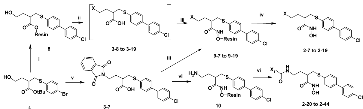
Scheme 4. Synthesis of compounds 2-7 to 2-44 . (i) (a) Ac_2O , pyridine, CH_2Cl_2 , rt, 18 h, (92%); (b) 4-ClPhSnBu_3 , Pd(PPh_3)_4 , LiCl , toluene, 80^\circ C , 12 h, (76%); (c) TFA, CH_2Cl_2 , rt, 48 h, (91.5%); (d) LiOH, H_2O/THF , 0^\circ C ; (e) HATU , DIEA , ( o -Cl-trityl)-resin; (ii) (a) PPh_3 , DIAD , XH , THF/CH_2Cl_2 , rt; (b) 5% TFA , CH_2Cl_2 , 0^\circ C -rt, 18 h ( 3-8 to 3-19 ); (iii) HATU , DIEA , hydroxylamine-resin; (iv) 5% TFA , CH_2Cl_2 ( 2-7 to 2-19 ); (v) (a) PPh_3 , DIAD , PhNH_2 , 0^\circ C -rt, 12 h, (99%); (b) 4-ClPhSnBu_3 , Pd(PPh_3)_4 , LiCl , toluene, 80^\circ C , 18 h, (62%); (c) TFA , CH_2Cl_2 , 0^\circ C -rt, 18 h, ( 3-7 , 100%); (vi) (a) HATU , DIEA , hydroxylamine-resin; (b) NH_2NH_2 , MeOH ; (vii) (a) X_1CO_2H , HATU , DIEA ; (b) 5% TFA , CH_2Cl_2 ( 2-20 to 2-44 ).
